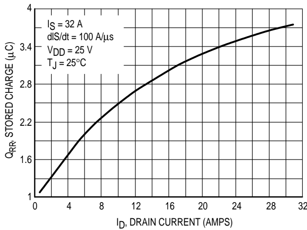
Figure 10. Stored Charge
