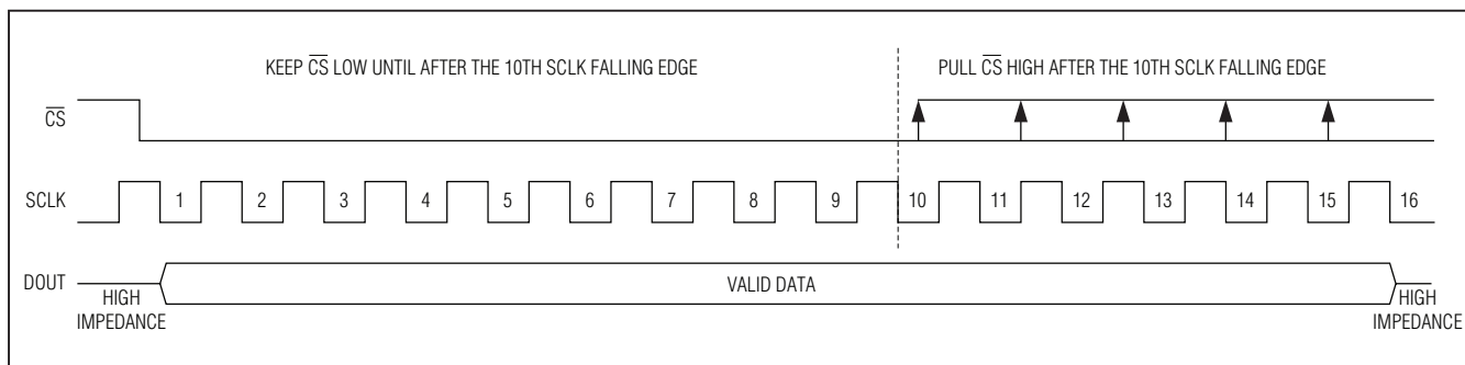
Figure 7. Normal Mode
