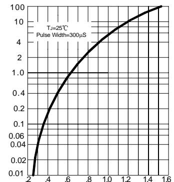
FIG.4 – TYPICAL FORWARD CHARACTERISTIC
