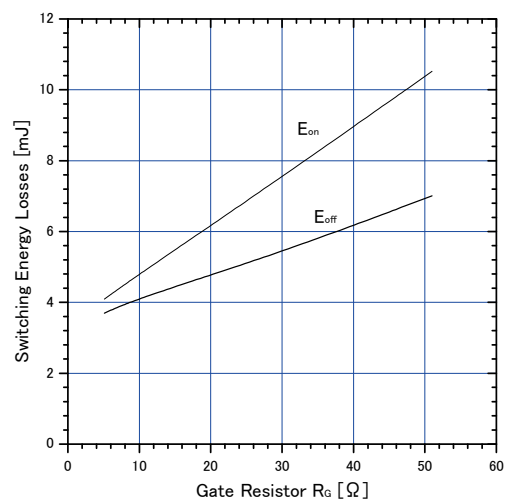
Graph.12 Typical switching losses vs. R_G T_J=175^{\circ}C, V_{CC}=400V, I_c=75A, L=500\mu H V_{GE}=15V
