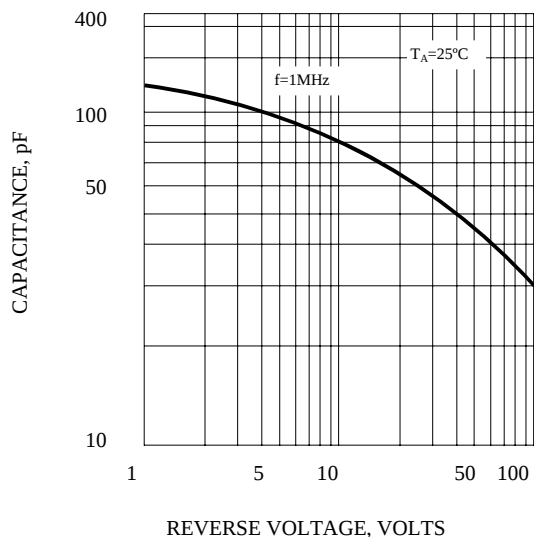
FIG. 3 - TYPICAL JUNCTION CAPACITANCE PER ELEMENT
