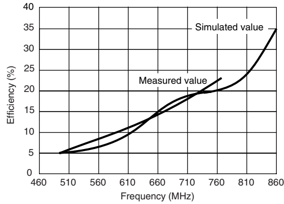
Figure 2. Radiation Efficiency vs. Frequency
