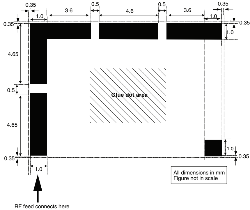
Figure 6. VJ 6040 Footprint
