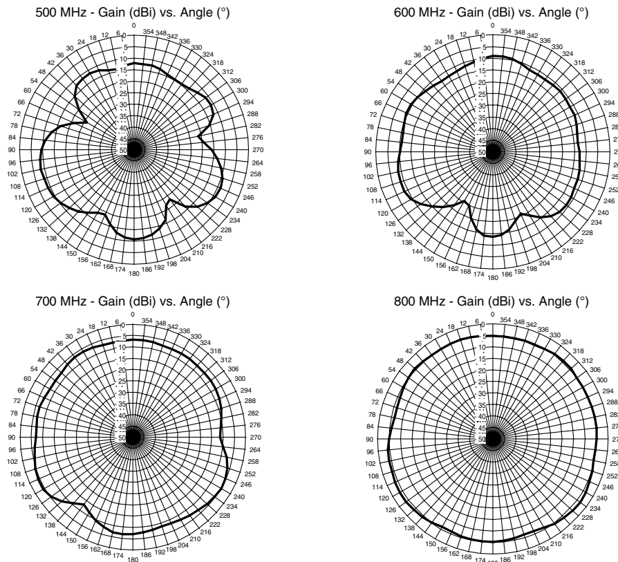
Figure 5. Measured Radiation Pattern
