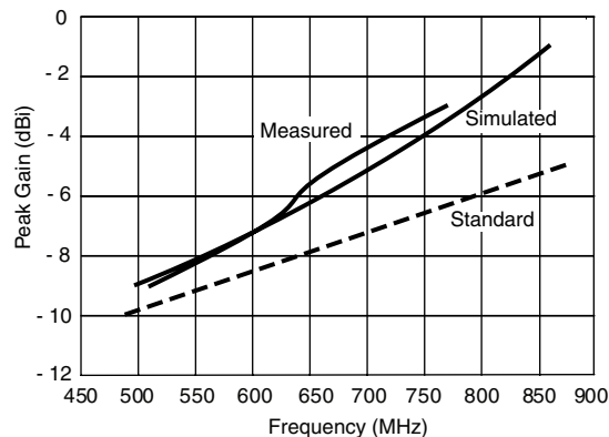
Figure 1. Peak Gain vs. Frequency
