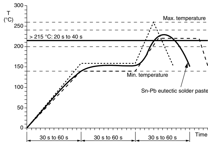
Figure 7. Soldering IR reflow with SnPb solder
