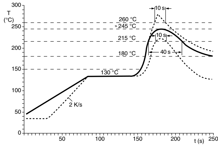
Figure 8. Soldering Reflow with Sn Solder
