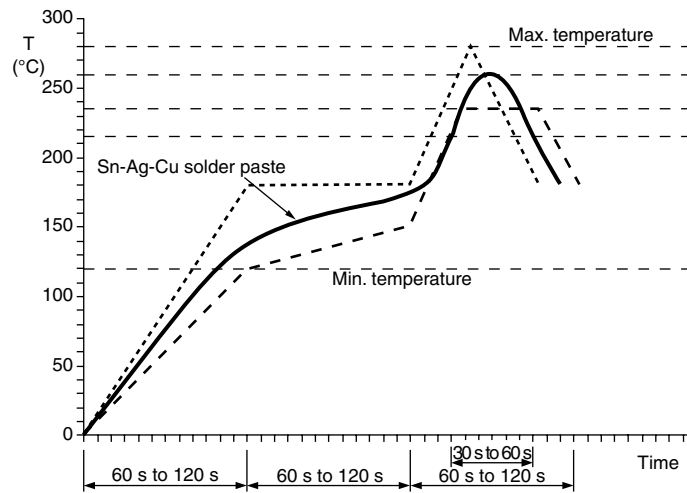
Figure 9. Soldering IR Reflow with SnAgCu Solder
