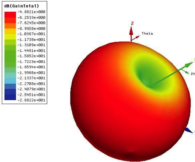
Figure 5. Simulated Radiation Pattern
