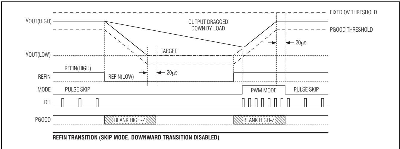
Figure 9. REFIN Transition (Skip Mode, Downward Transition Disabled)
