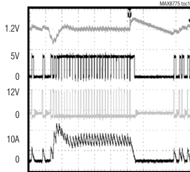
LOAD TRANSIENT (SEPARATE MODE)
