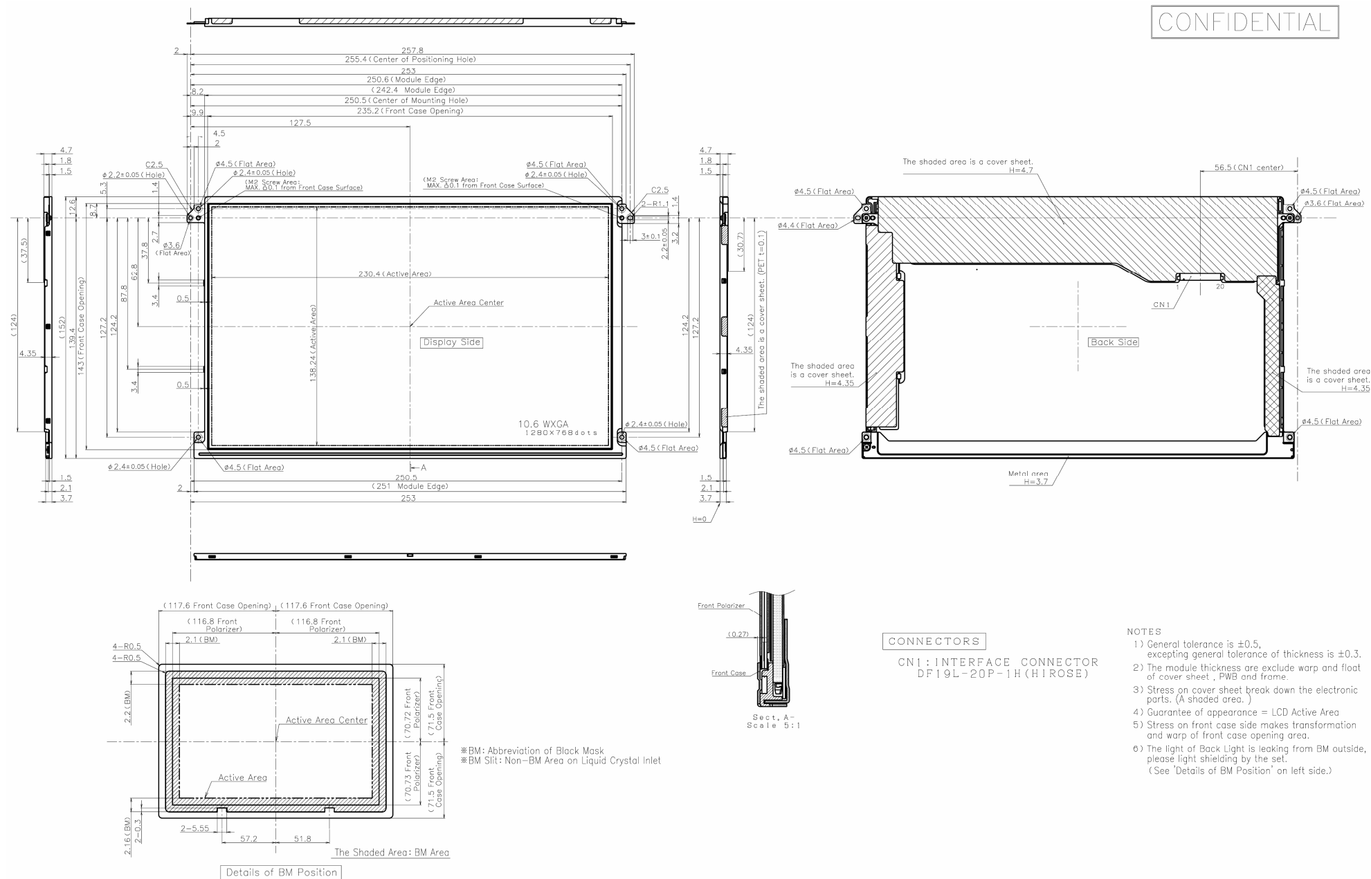
Fig.2 Outline Dimensions
