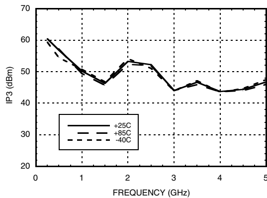
Input IP3 * @ 5V
