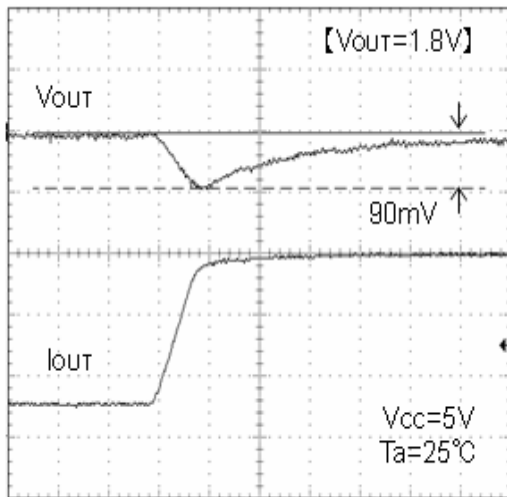
Fig.16 Transient response I_o=100 \rightarrow 600mA(10\mu s)
