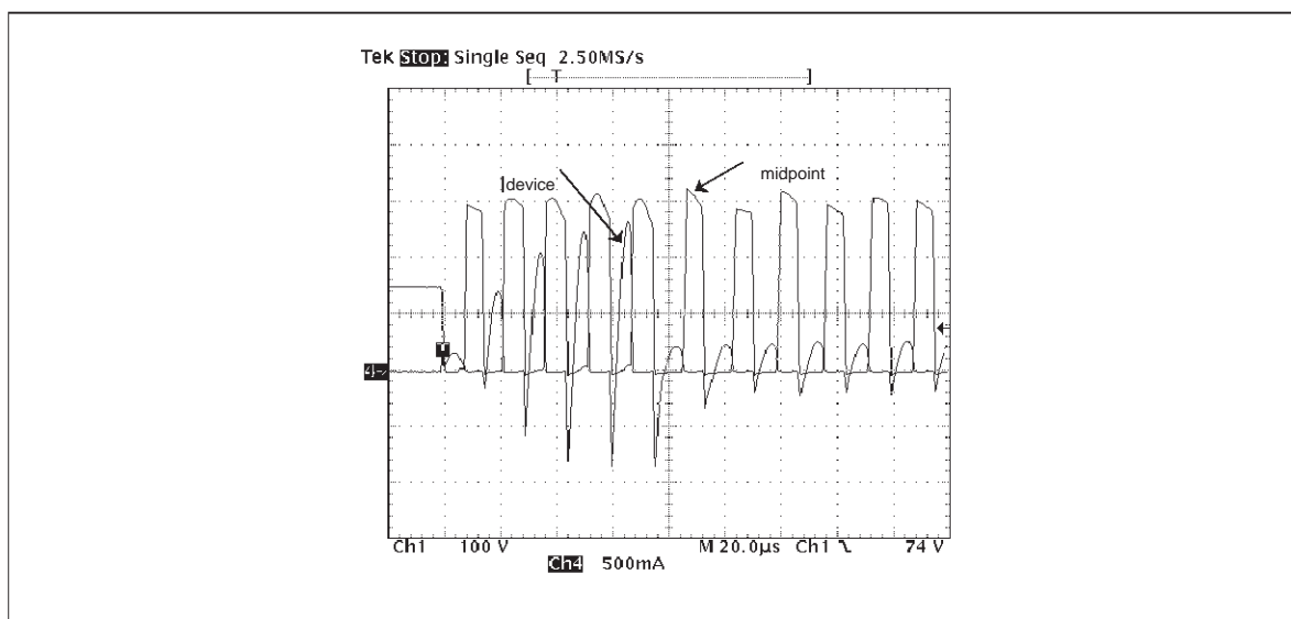
Figure 2: Start-up phase
