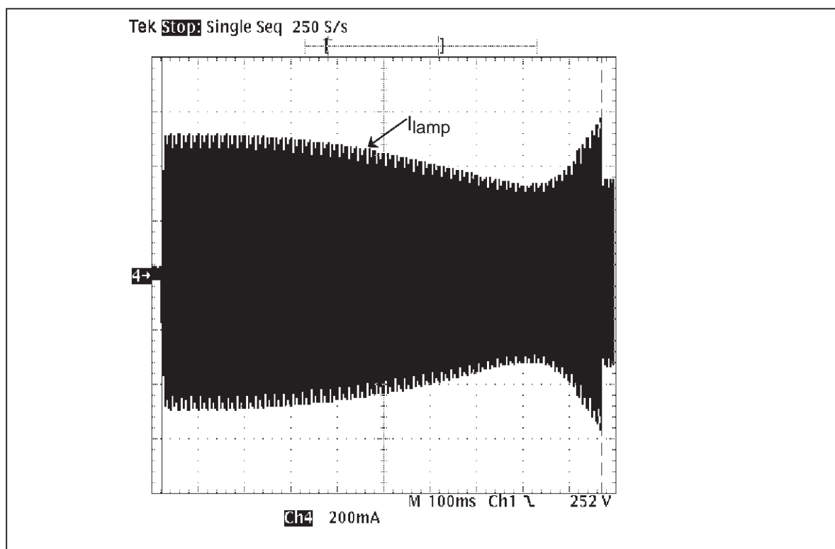
Figure 5: Pre-heating phase
