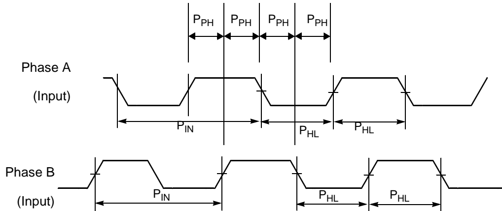
Figure 26. Quadrature Decoder Timing
