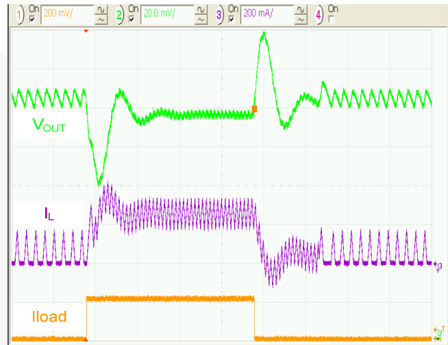
Figure 14. Load Transient 50 to 250mA, 3.6V IN , 5 \mu s /div.
