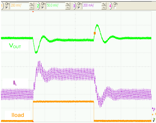
Figure 15. Load Transient 200 to 500mA, 3.6V IN , 5 \mu s /div.
