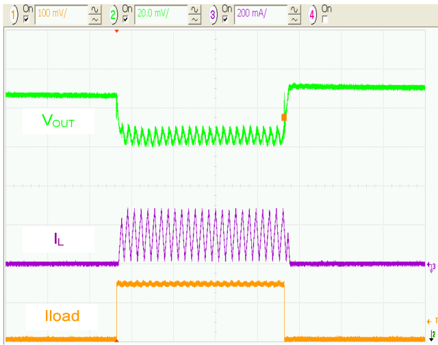
Figure 13. Load Transient 0 to 150mA, 3.6V IN , 5 \mu s /div.
