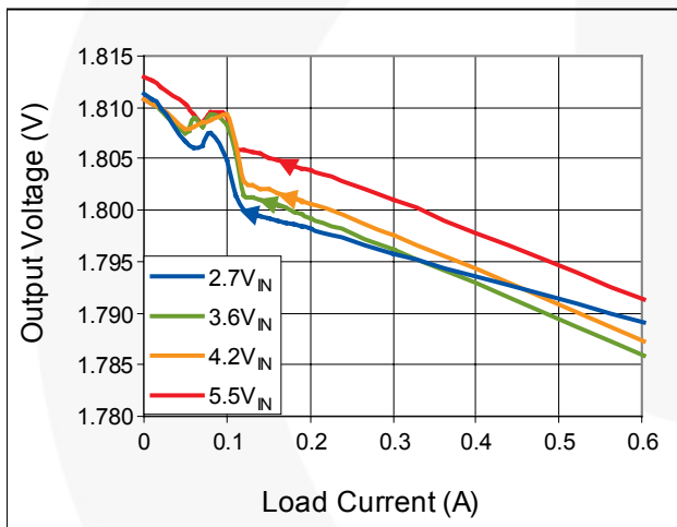
Figure 6. Voltage Regulation
