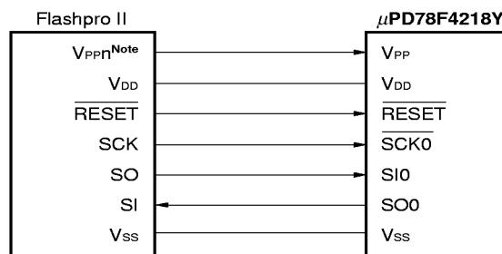
Figure 7-2. Connection of Flashpro II in 3-Wire Serial I/O Mode (when using 3-wire serial I/O)
