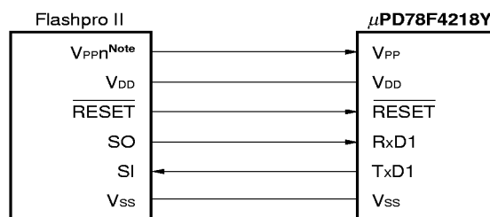
Figure 7-3. Connection of Flashpro II in UART Mode (when using UART1)
