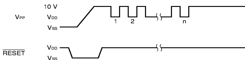
Figure 7-1. Communication Mode Selecting Format
