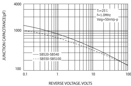
FIG.5-TYPICAL JUNCTION CAPACITANCE
