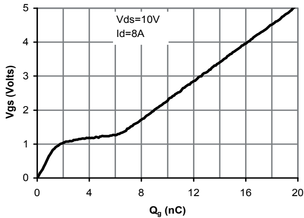
Figure 7: Gate-Charge Characteristics
