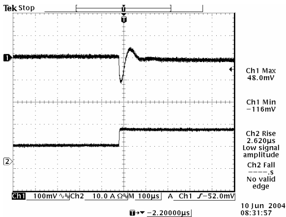
50% to 100% load step at Vin=5.0 V, Vo=3.3 V
