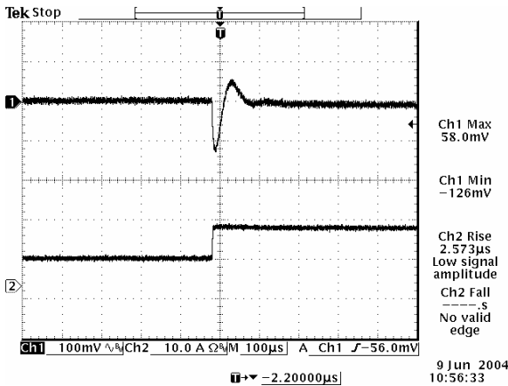
50% to 100% load step at Vin=5.0 V, Vo=1.8 V
