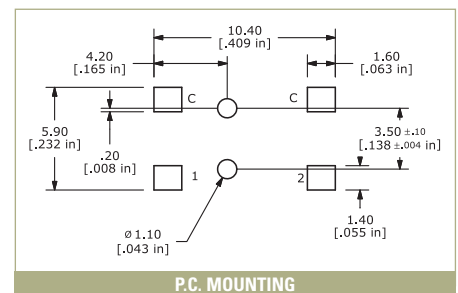
P.C. MOUNTING
