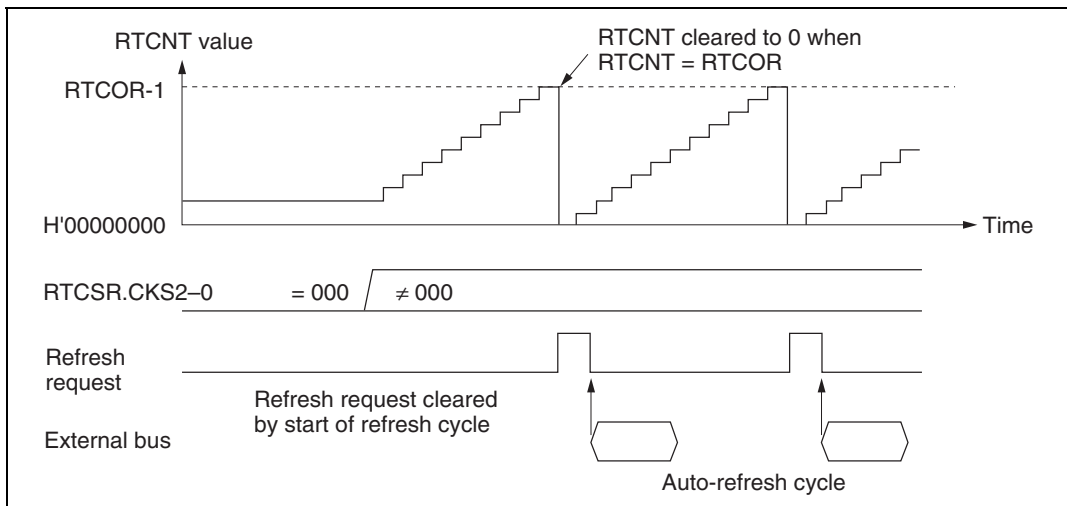
Figure 13.35 Auto-Refresh Operation
