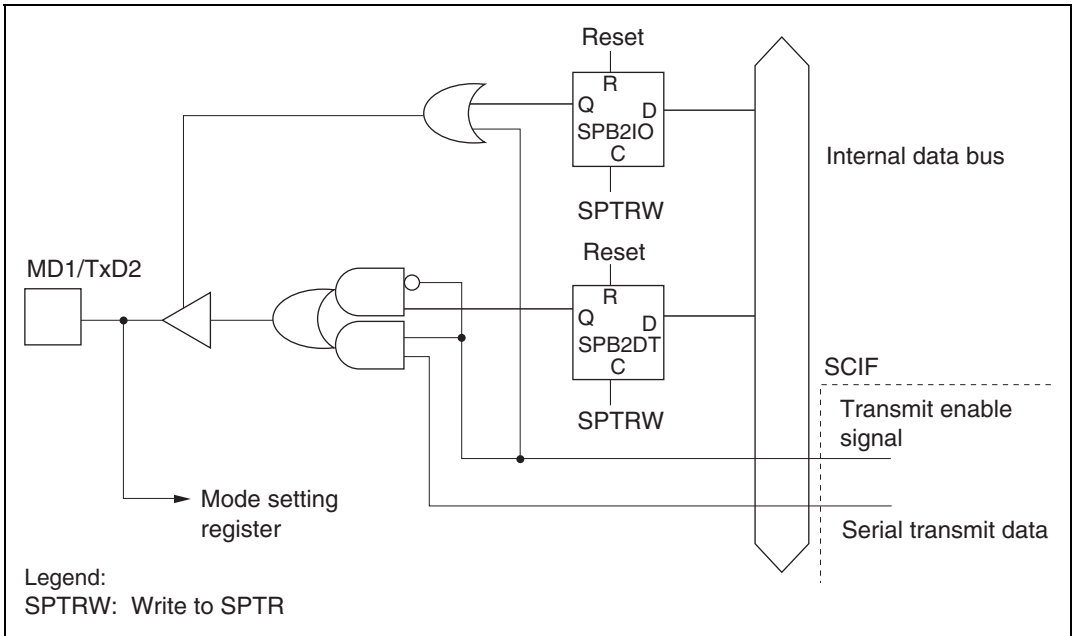
Figure 18.6 MD1/TxD2 Pin
