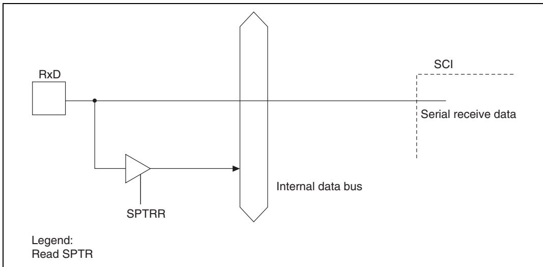
Figure 18.5 RxD Pin
