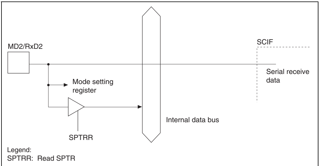
Figure 18.7 MD2/RxD2 Pin
