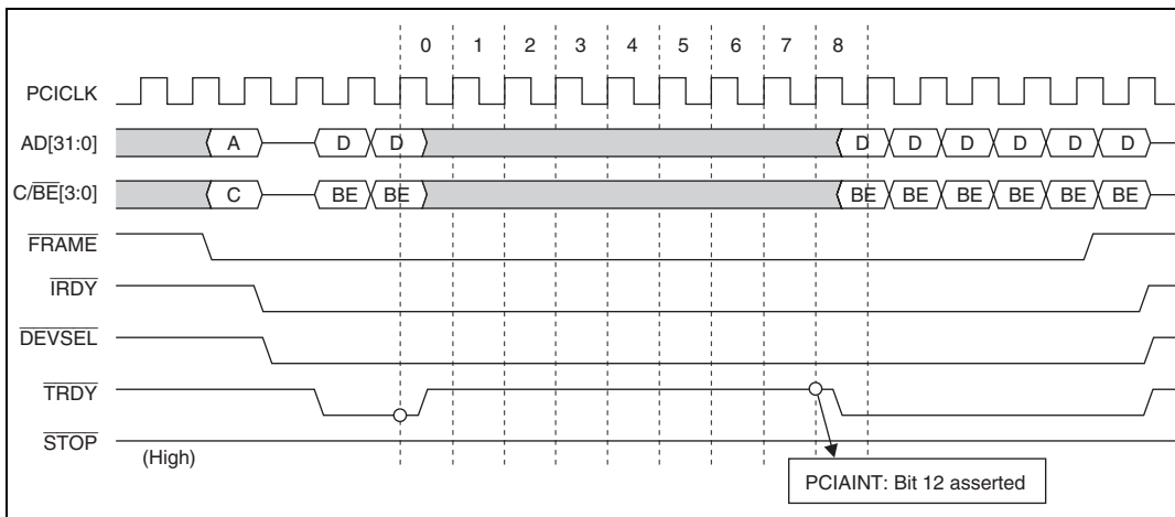
Figure 22.25 Target Bus Timeout Interrupt Generation Example 2 (Example in which the Target Device Takes 8 Clock Cycles to Prepare for the Third Data Transfer)
