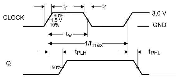
Figure 1. Switching Waveforms
