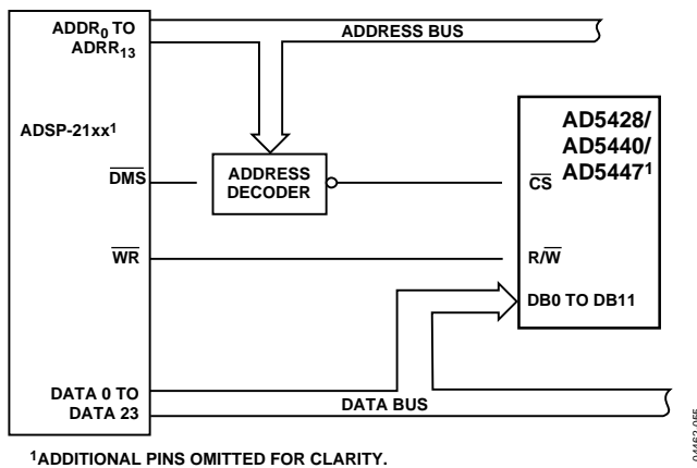
Figure 44. ADSP21xx-to-AD5428/AD5440/AD5447 Interface
