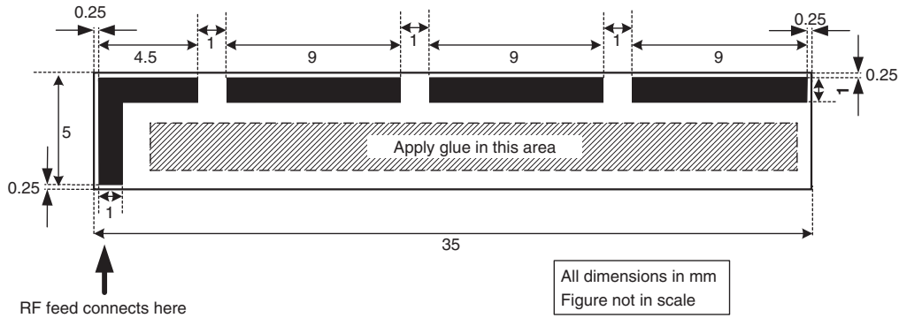
Figure 4. VJ 3505 Footprint
