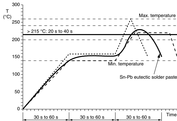
Figure 5. Soldering IR reflow with SnPb solder
