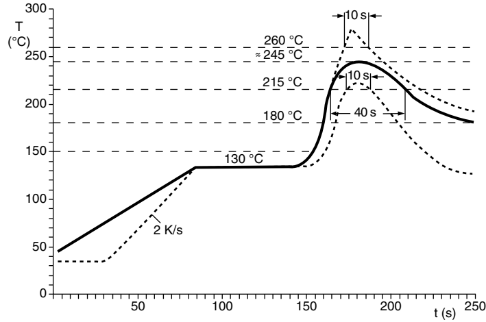
Figure 6. Soldering Reflow with Sn Solder
