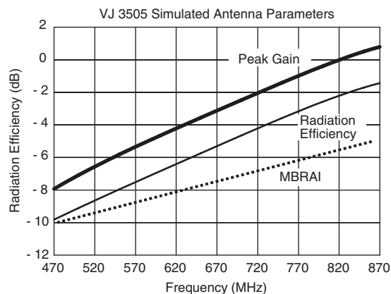
Figure 1. Peak Gain and Efficiency vs. Frequency
