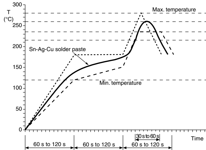
Figure 7. Soldering IR Reflow with SnAgCu Solder
