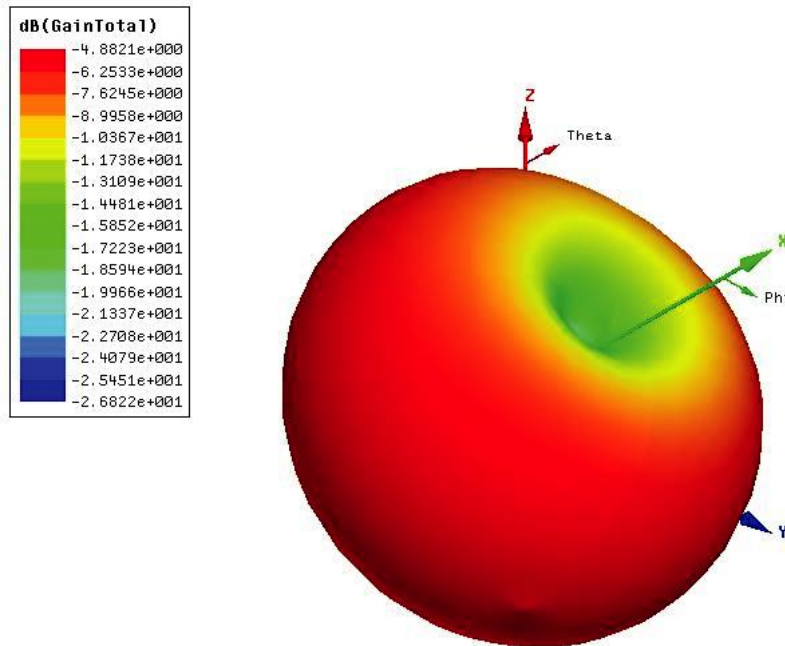
Figure 3. Simulated Radiation Pattern at 550 MHz
