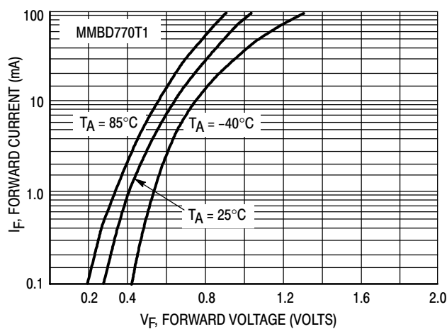
Figure 8. Forward Voltage
