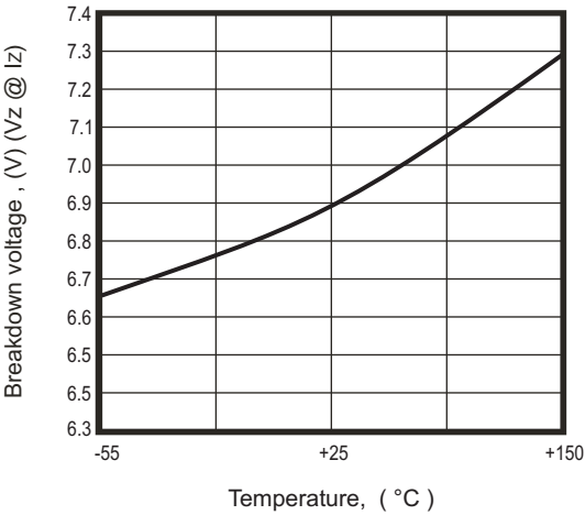
Fig. 1 - Typical breakdown votage versus temperature
