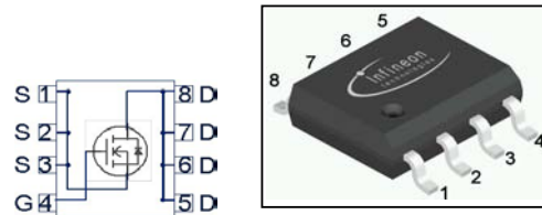
PG-DSO-8
