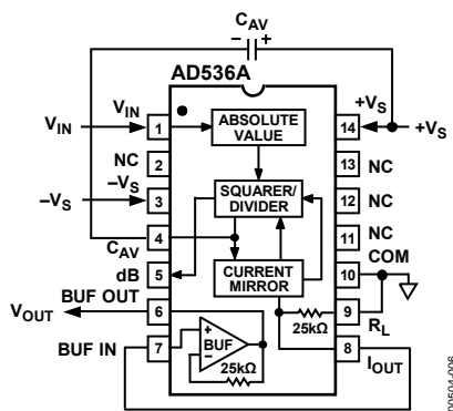
Figure 6. 14-Lead Standard RMS Connection
