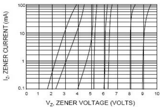
FIG. 7 - ZENER VOLTAGE VS. ZENER CURRENT V Z = 3.3 thru 10 VOLTS
