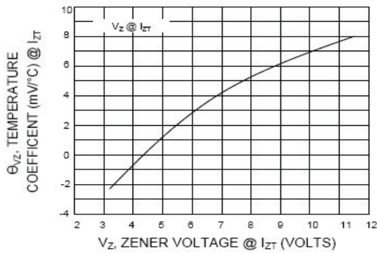
FIG. 5 - TEMPERATURE COEFFICIENT RANGES UNITS TO 12 VOLTS
