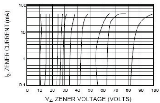
FIG. 8 - ZENER VOLTAGE VS. ZENER CURRENT V Z = 12 thru 82 VOLTS
