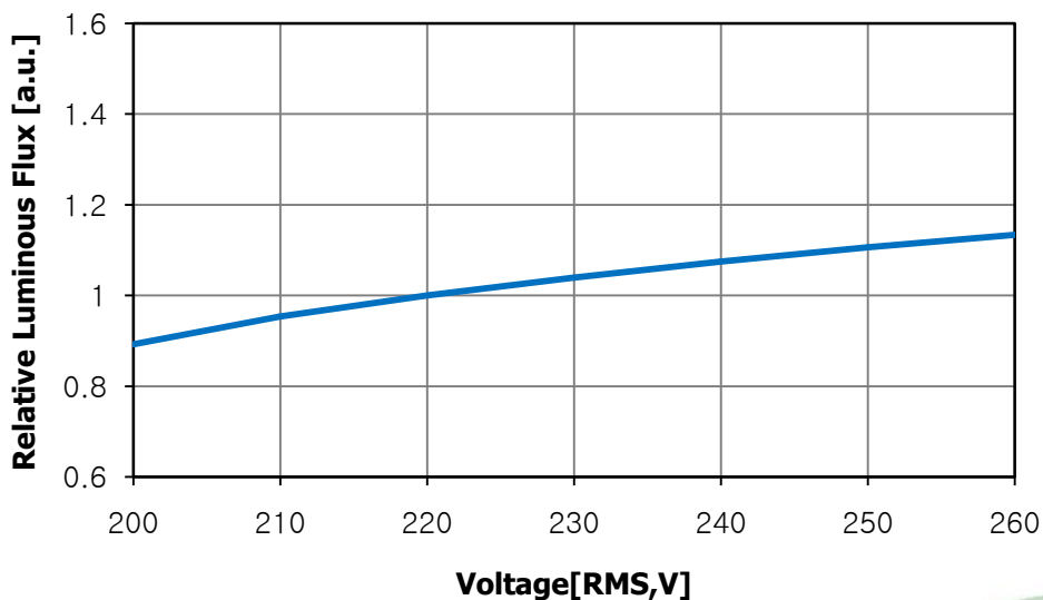
Relative Luminous flux vs. Forward Voltage, Ta= 25°C
