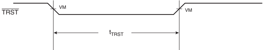
Figure 9-6. TRST Timing Diagram
