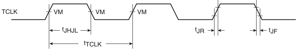
Figure 9-5. JTAG Clock Input Timing Diagram
