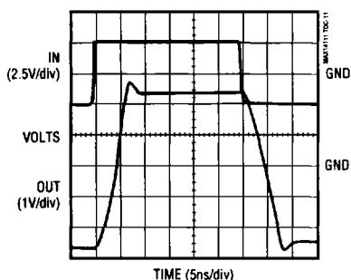
LARGE-SIGNAL PULSE RESPONSE ( R_L = 5k\Omega )
