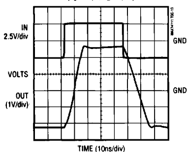
LARGE-SIGNAL PULSE RESPONSE ( C_L = 47pF , R_L = \text{open} )
