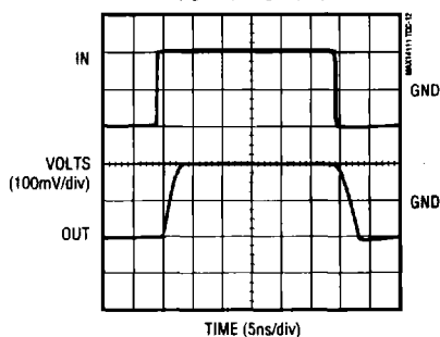
SMALL-SIGNAL PULSE RESPONSE ( C_L = 47pF , R_L = \text{open} )
