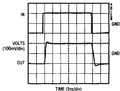
SMALL-SIGNAL PULSE RESPONSE ( R_L = 5k\Omega )
