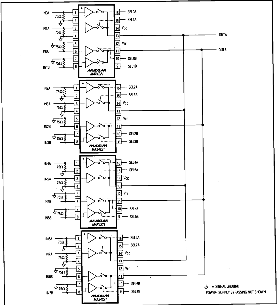
Figure 6. 8x2 Multiplexer Using MAX4221
