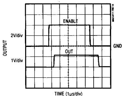
ENABLE/DISABLE DELAY TIME (INPUT = 1.1V)
