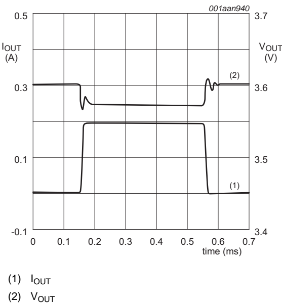
Fig 28. Load regulation for LD6806F/36H
