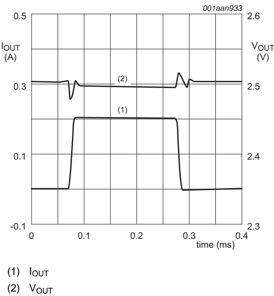
Fig 25. Load regulation for LD6806CX4/25H
