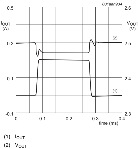
Fig 26. Load regulation for LD6806F/25H
