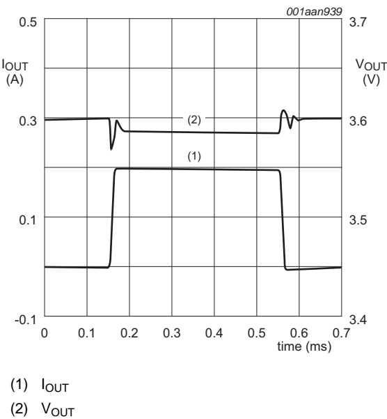
Fig 27. Load regulation for LD6806CX4/36H
