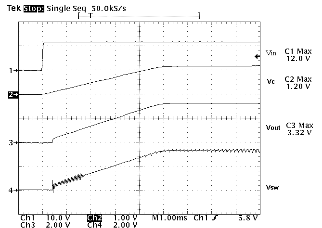
Figure 8. The Power Up Transition of NCV8842 Regulator
