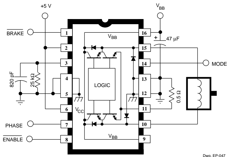
Typical DC Servo Motor Application
