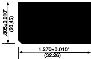
TOPVIEW - "A" Package Option
