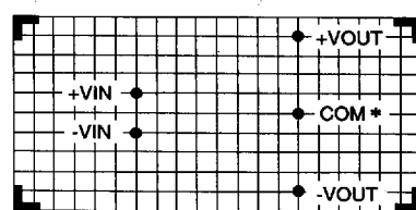
BOTTOMVIEW - "B" Package Option
