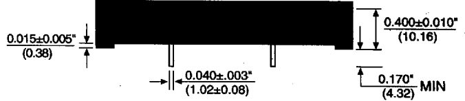
SIDEVIEW - "B" Package Option
