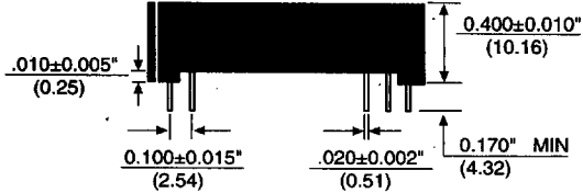
SIDEVIEW - "A" Package Option
