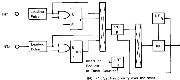
Figure 20 Interrupt Circuit Block Diagram
