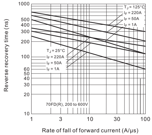
Fig.6 Typical reverse recovery time vs. rate of fall of forward current.
