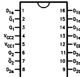
16-Pin Flatpak
