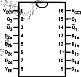
16-Pin DIP
