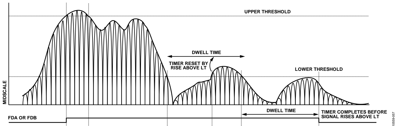
Figure 57. Threshold Settings for FDA and FDB Signals
