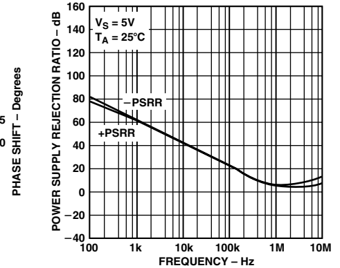
TPC 15. Power Supply Rejection Ratio vs. Frequency
