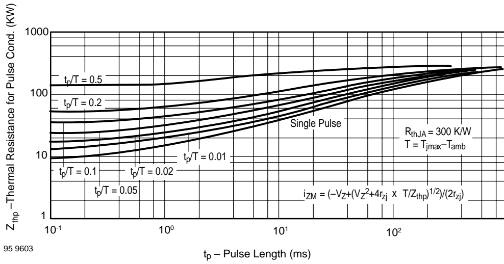
Figure 11. Thermal Response
