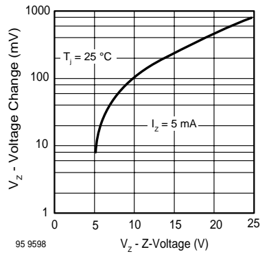
Figure 2. Typical Change of Working Voltage under Operating Conditions at T_{amb} = 25\text{ °C}
