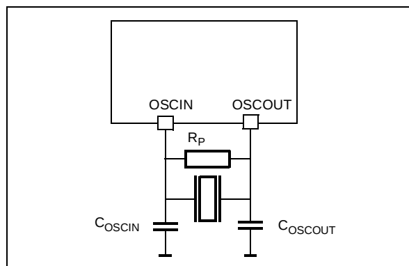
Figure 10. Crystal/Ceramic Resonator
