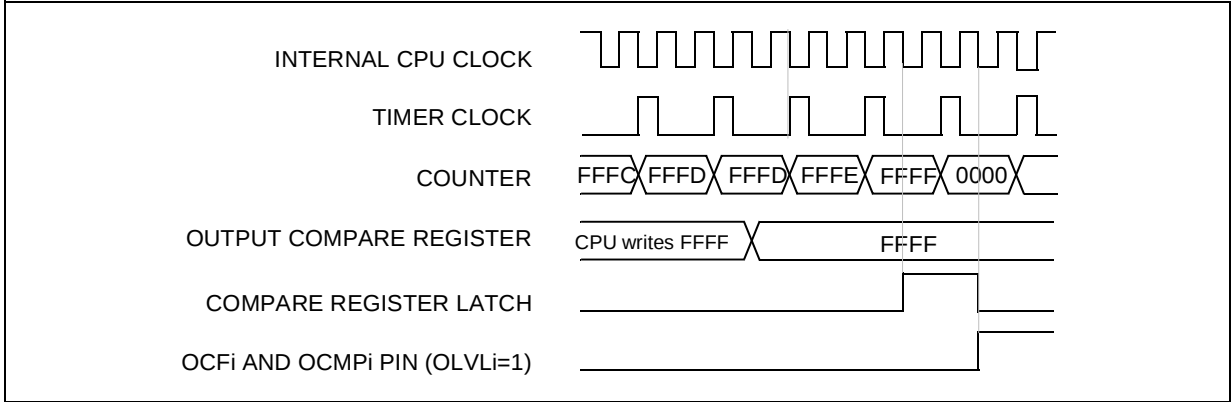
Figure 29. Output Compare Timing Diagram, Internal Clock Divided by 2
