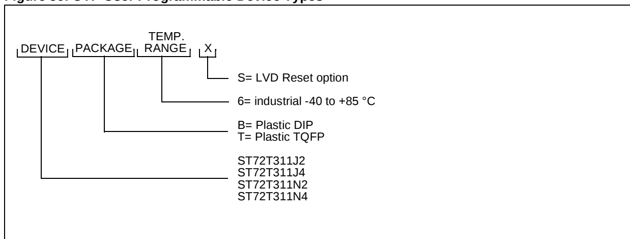
Figure 59. OTP User Programmable Device Types
