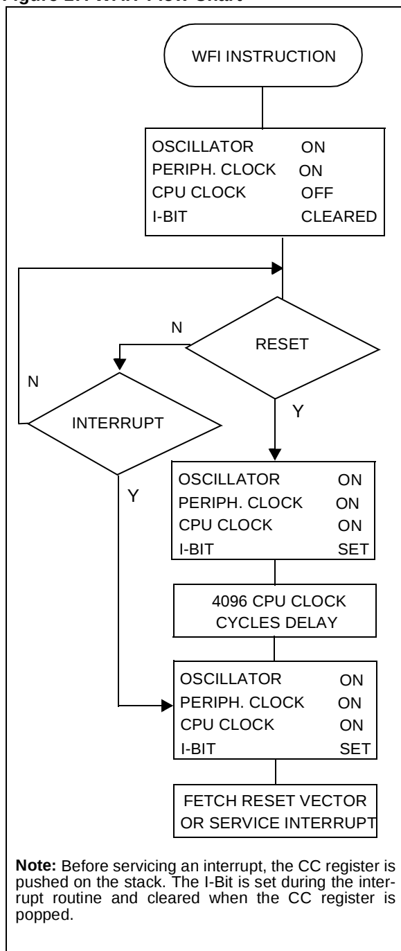
Figure 17. WAIT Flow Chart
