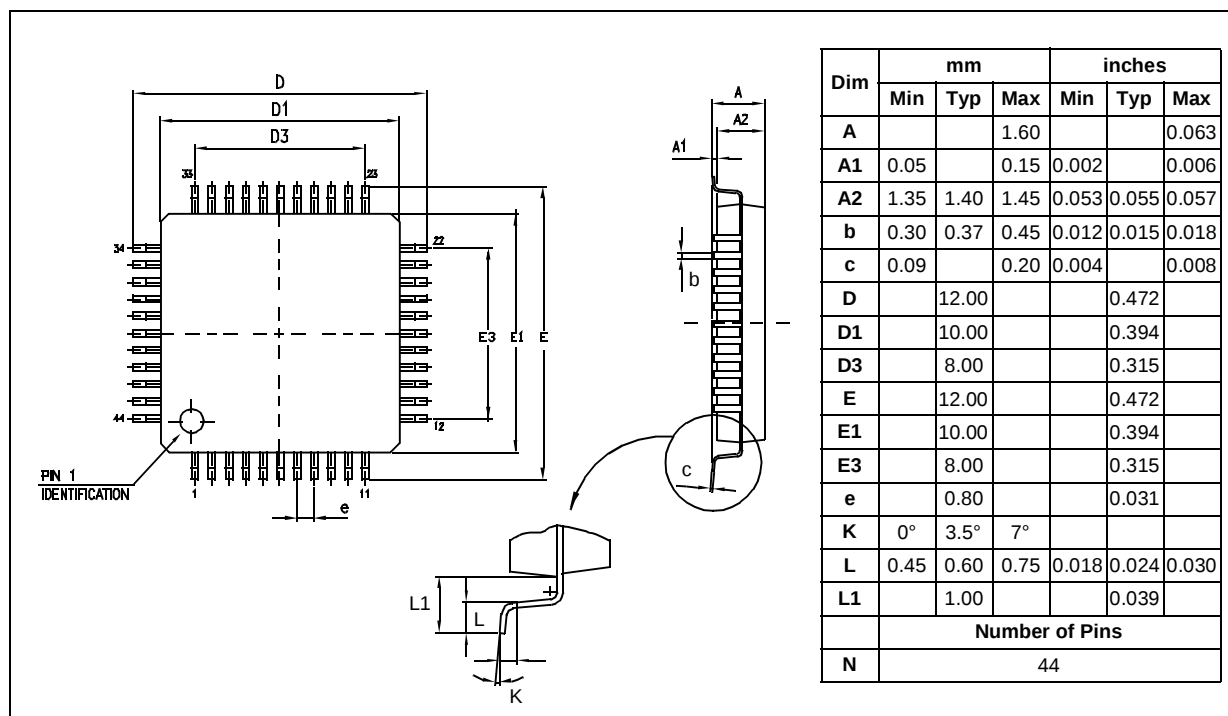
Figure 57. 44-Pin Thin Quad Flat Package
