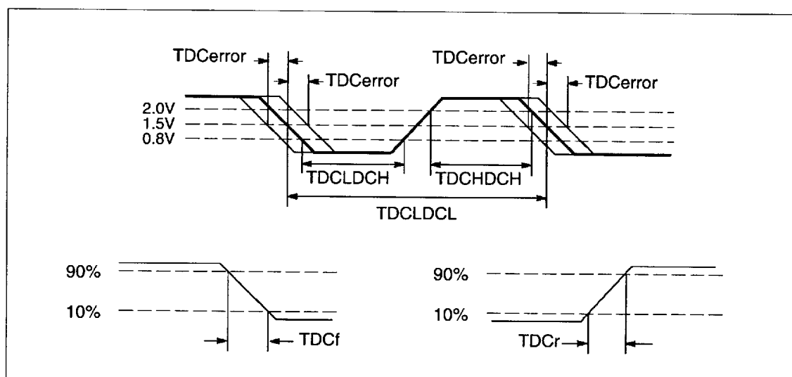
Figure 3.2 ClockIn timing
