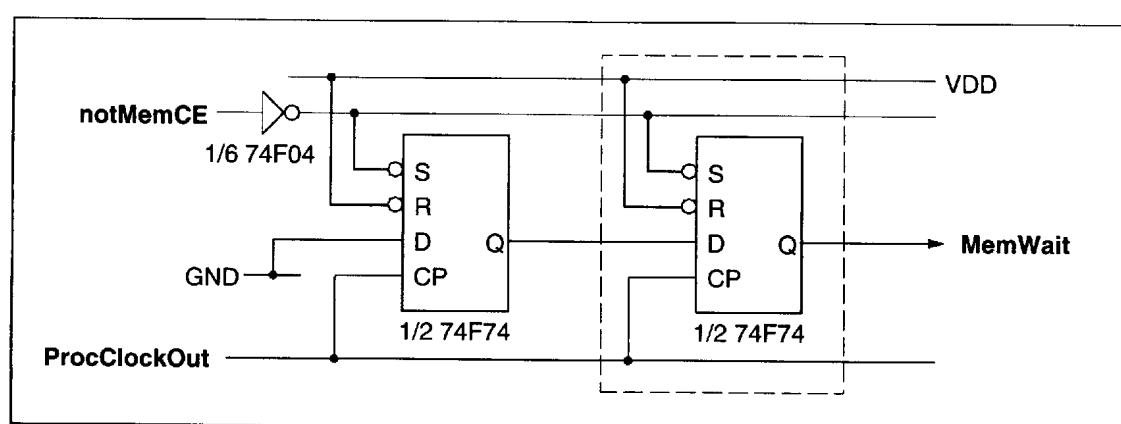
Figure 5.11 Extendable wait state generator
