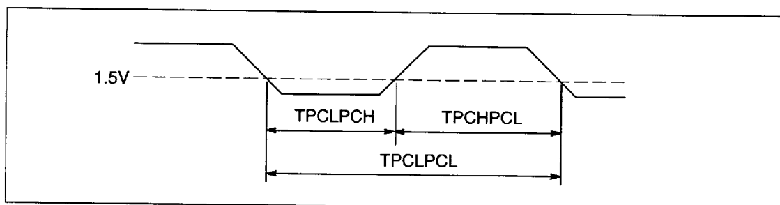
Figure 5.3 IMS T225 ProcClockOut timing
