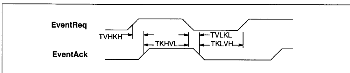
Figure 6.1 IMS T225 event timing
