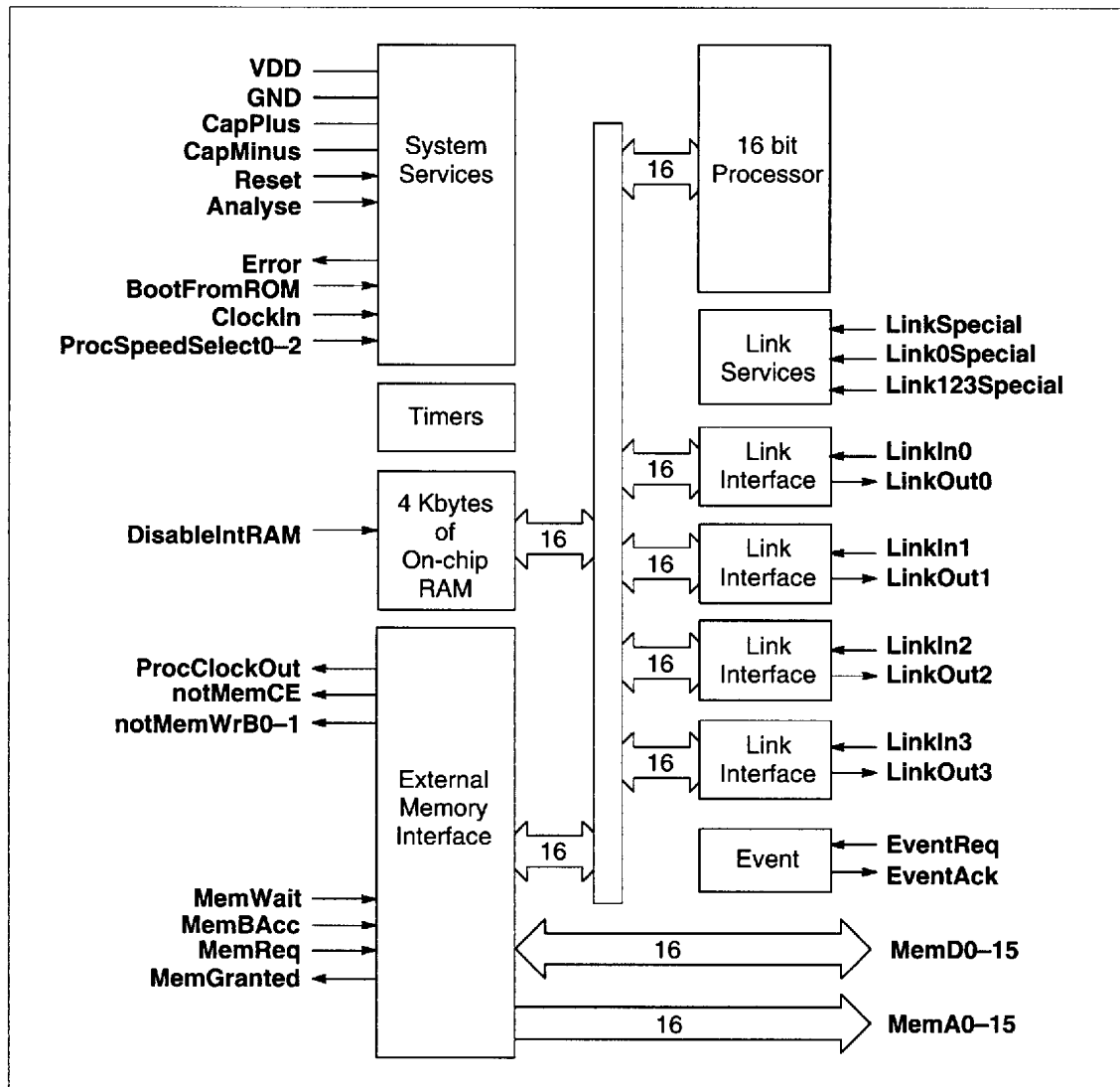
Figure 1.1 IMS T225 block diagram
