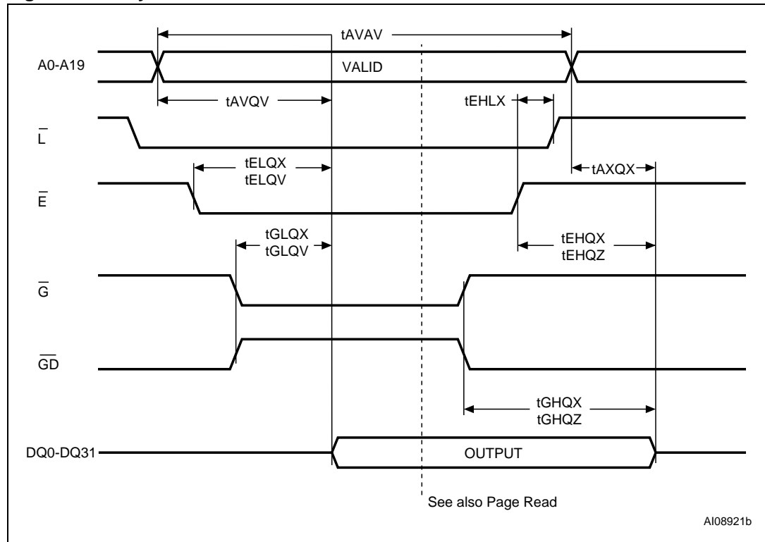
Figure 7. Asynchronous Bus Read AC waveforms
