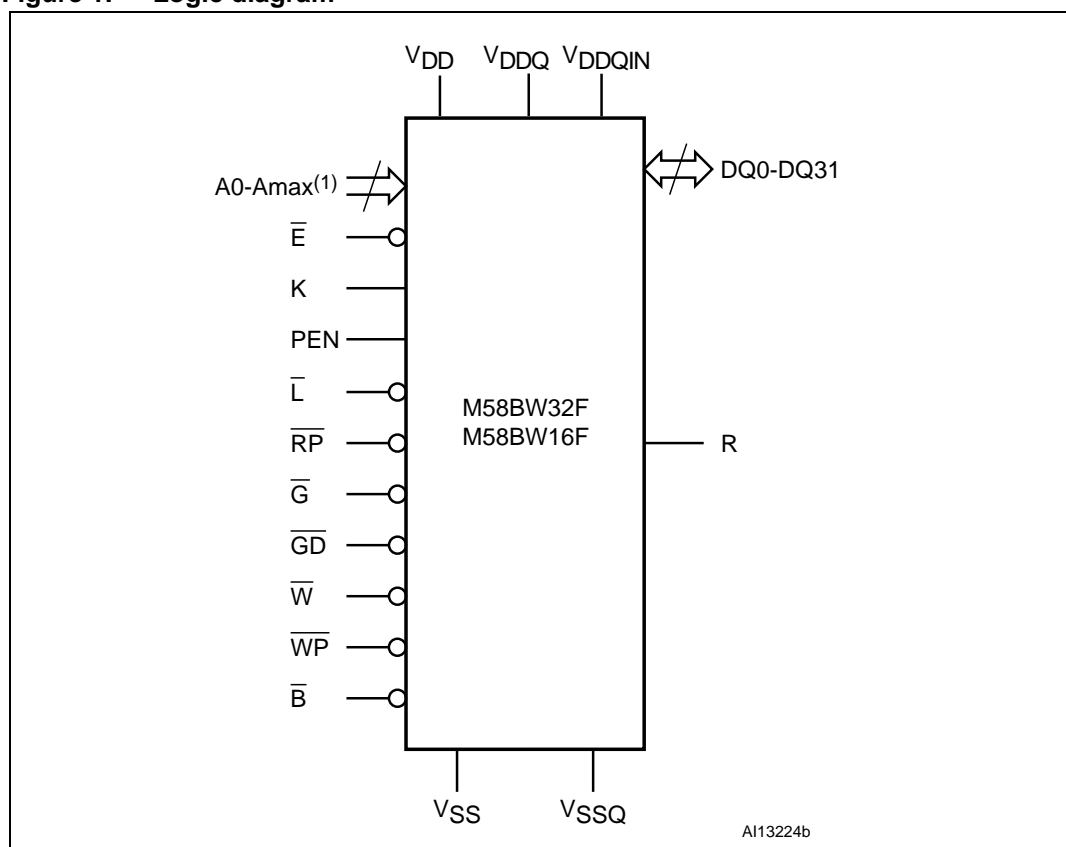
Figure 1. Logic diagram
