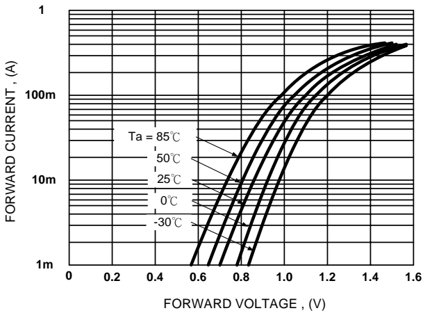
Figure 1. Forward Characteristics
