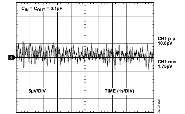
Figure 24. ADR121 0.1 Hz to 10 Hz Noise
