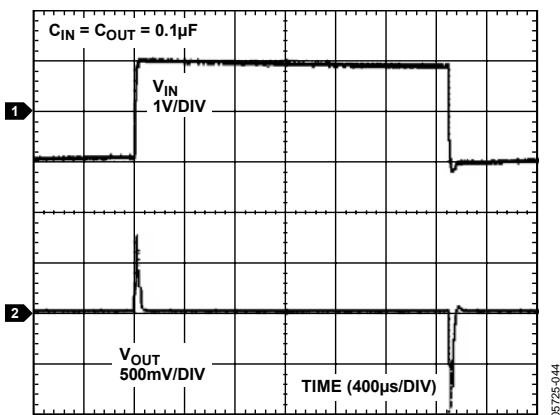
Figure 40. ADR125 Line Transient Response
