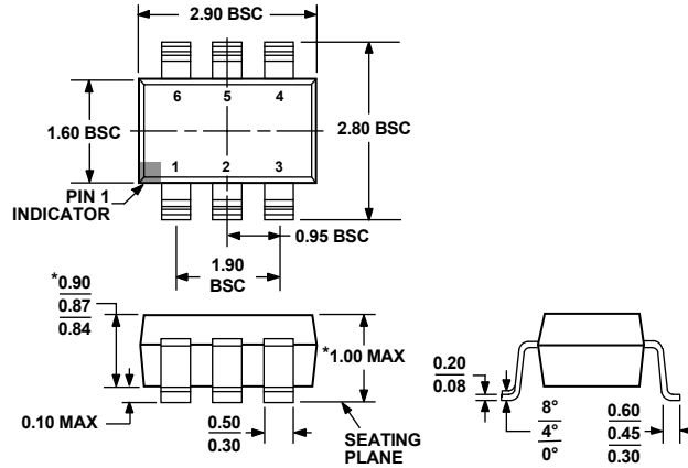
Figure 53. 6-Lead Thin Small Outline Transistor Package [TSOT]
