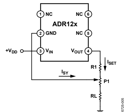
Figure 52. ADR12x Trim Configuration
