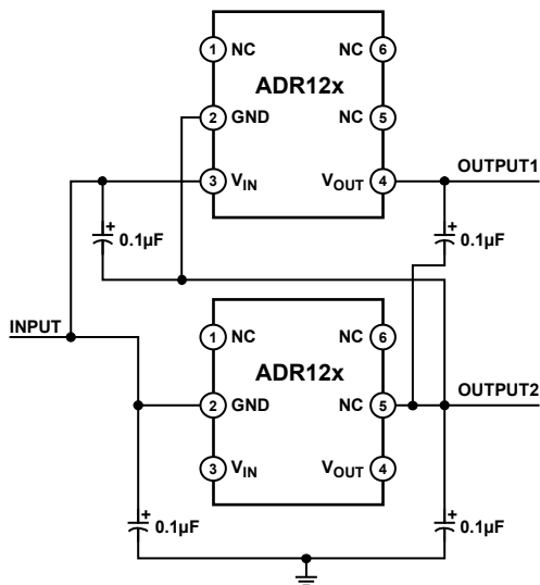
Figure 50. Stacking References with ADR12x
