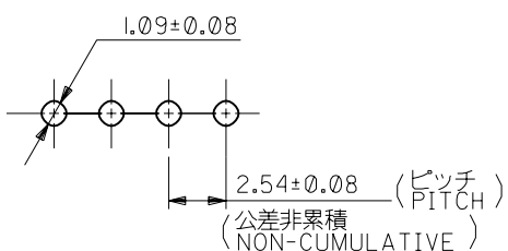
推奨基板穴寸法 RECOMMENDED P.C.B. LAYOUT
