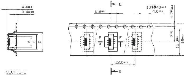
SECT. E-E
