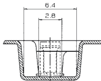
SECT. F-F
