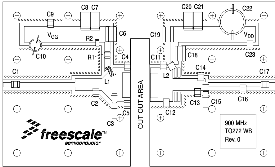
Figure 2. MRF6S9125NR1(NBR1)/MR1(MBR1) Test Circuit Component Layout
