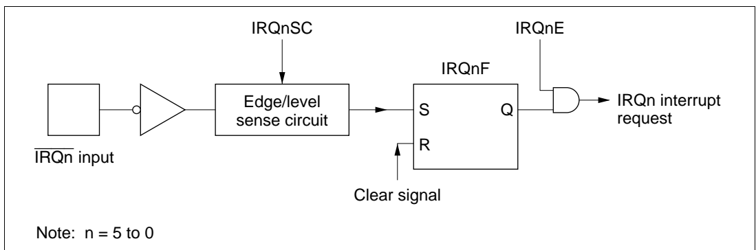
Figure 5.2 Block Diagram of Interrupts \text{IRQ}_0 to \text{IRQ}_5
