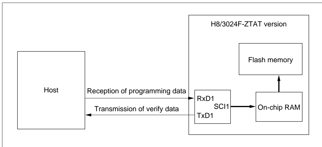
Figure 18.6 System Configuration When Using Boot Mode
