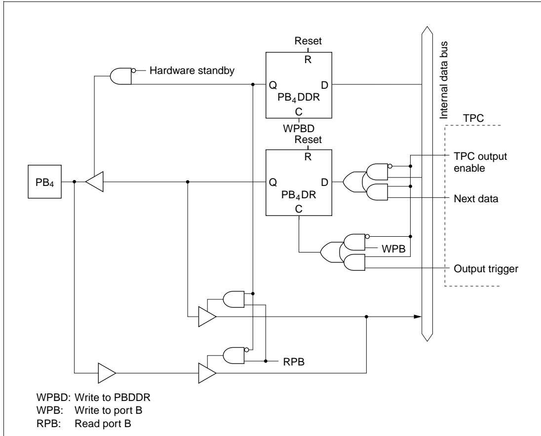
Figure C.11 (c) Port B Block Diagram (Pin PB 4 )
