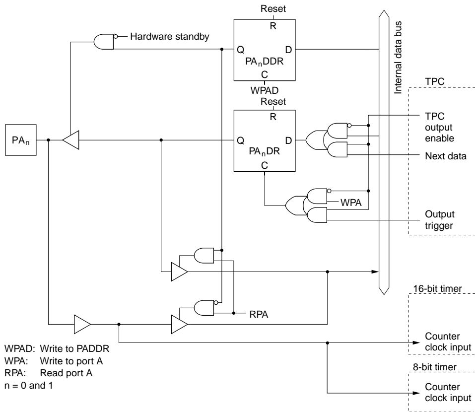
Figure C.10 (a) Port A Block Diagram (Pins PA 0 and PA 1 )
