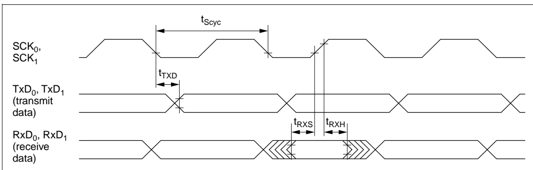
Figure 21.19 SCI Input/Output Timing in Synchronous Mode
