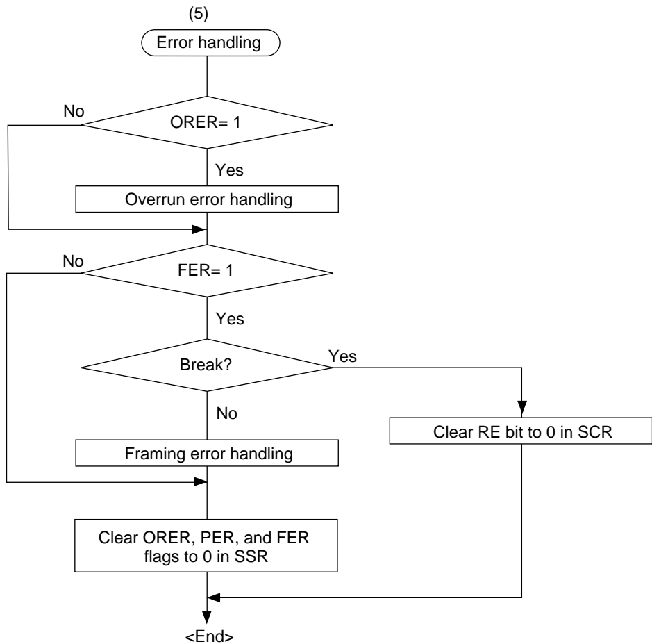
Figure 12.12 Sample Flowchart for Receiving Multiprocessor Serial Data (cont)
