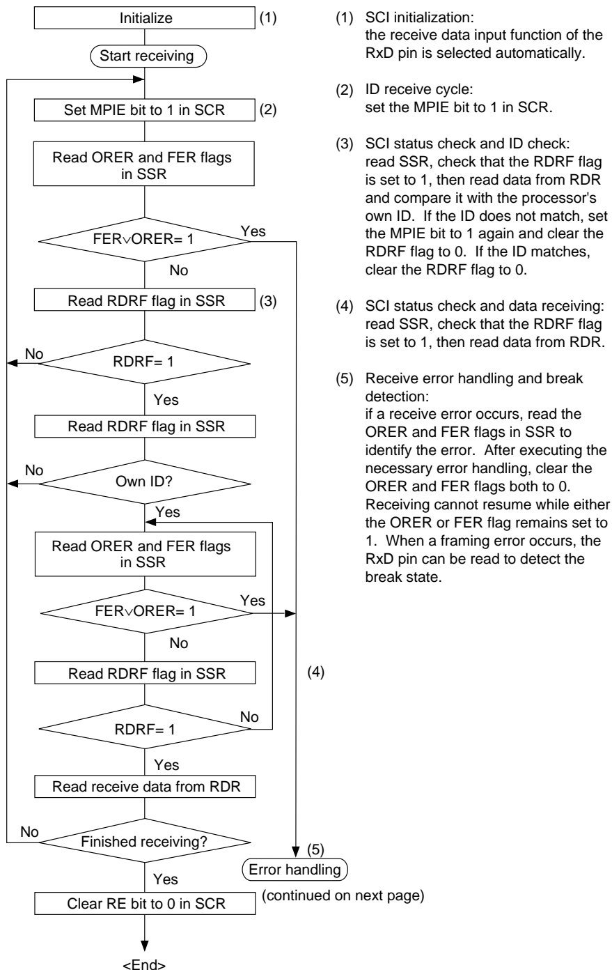
Figure 12.12 Sample Flowchart for Receiving Multiprocessor Serial Data
