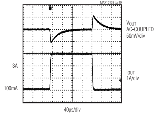
3A LOAD-TRANSIENT RESPONSE
